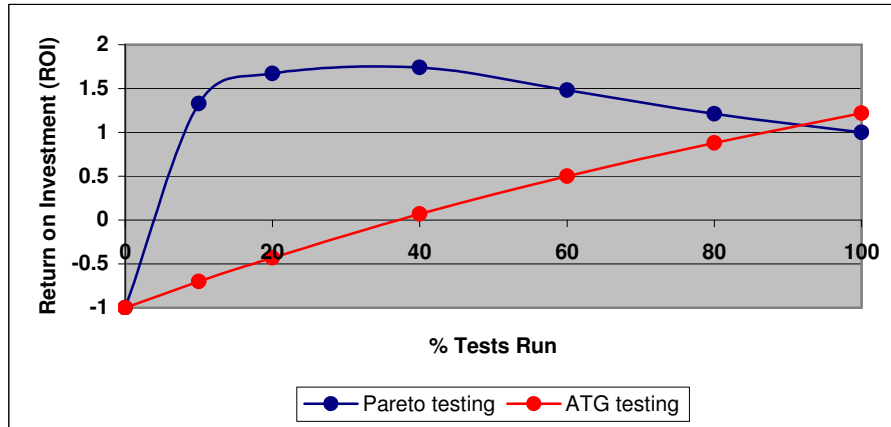
Figure 21.2 ROI: Value-Neutral ATG vs. Pareto Analysis
