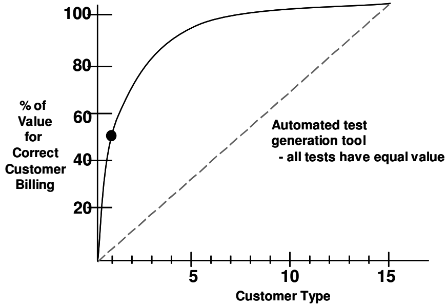
Figure 21.1 Pareto 80-20 distribution of test case value
